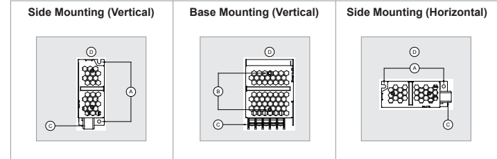
Fig. 2. Mounting Orientation
