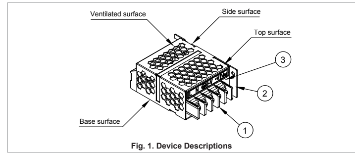
Fig. 1. Device Descriptions
