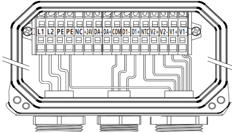
RDM/DMX Connection
