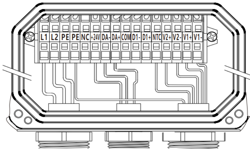
DALI Connection
