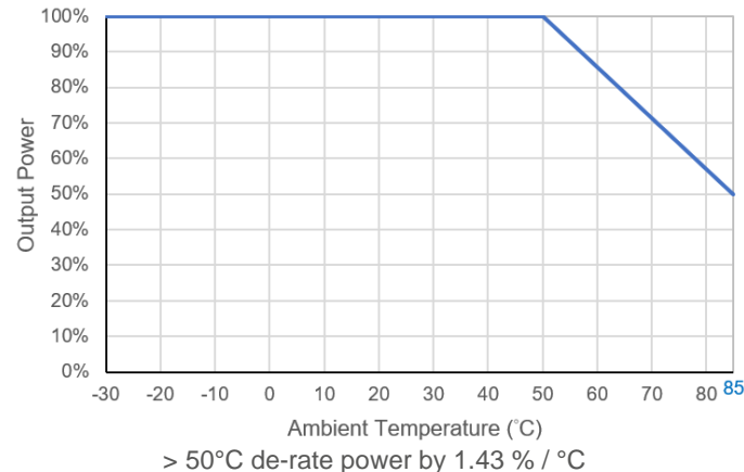
Power De-rating Curve (Force Air)
