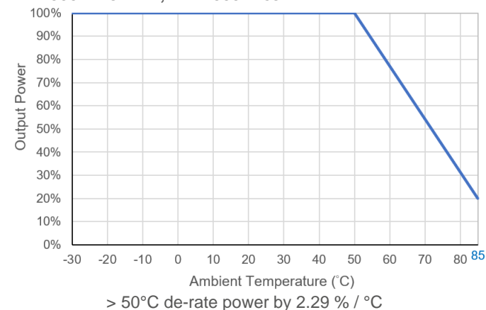
12V Fan Power De-rating Curve (Convection)
