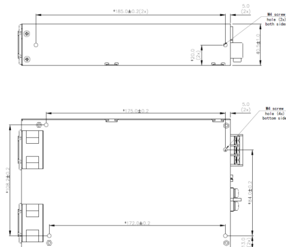
Fig. 4 Assembly Reference
