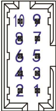
Fig. 4: Signal port and Auxiliary DC Output (CN604)
