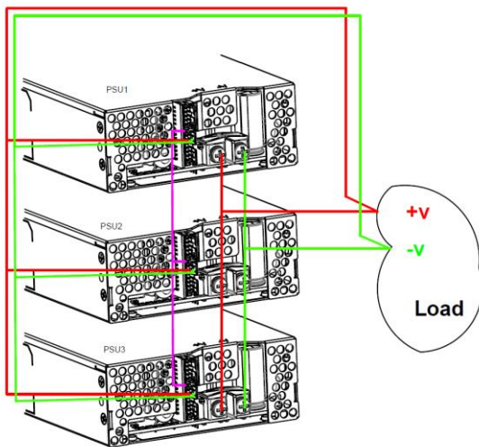
Fig. 24: parallel connection with remote sense
