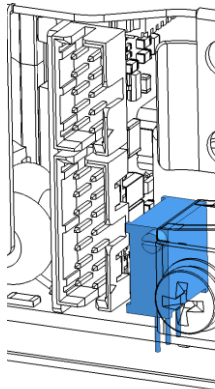
Fig. 7: Output voltage adjustment potentiometer
