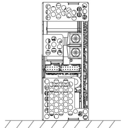
Fig. 12: Mounting on the left side
