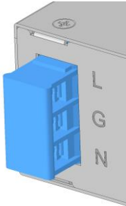
Fig. 2: AC/DC Input terminal block – pin assignment
