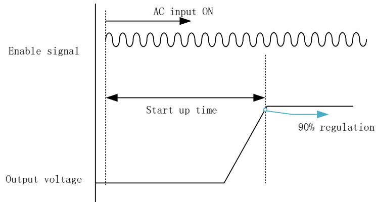
Fig. 15: Start-up timing sequence
