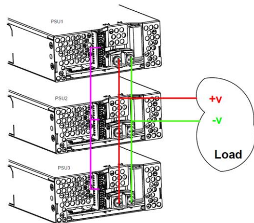
Fig. 25: parallel connection without remote sens
