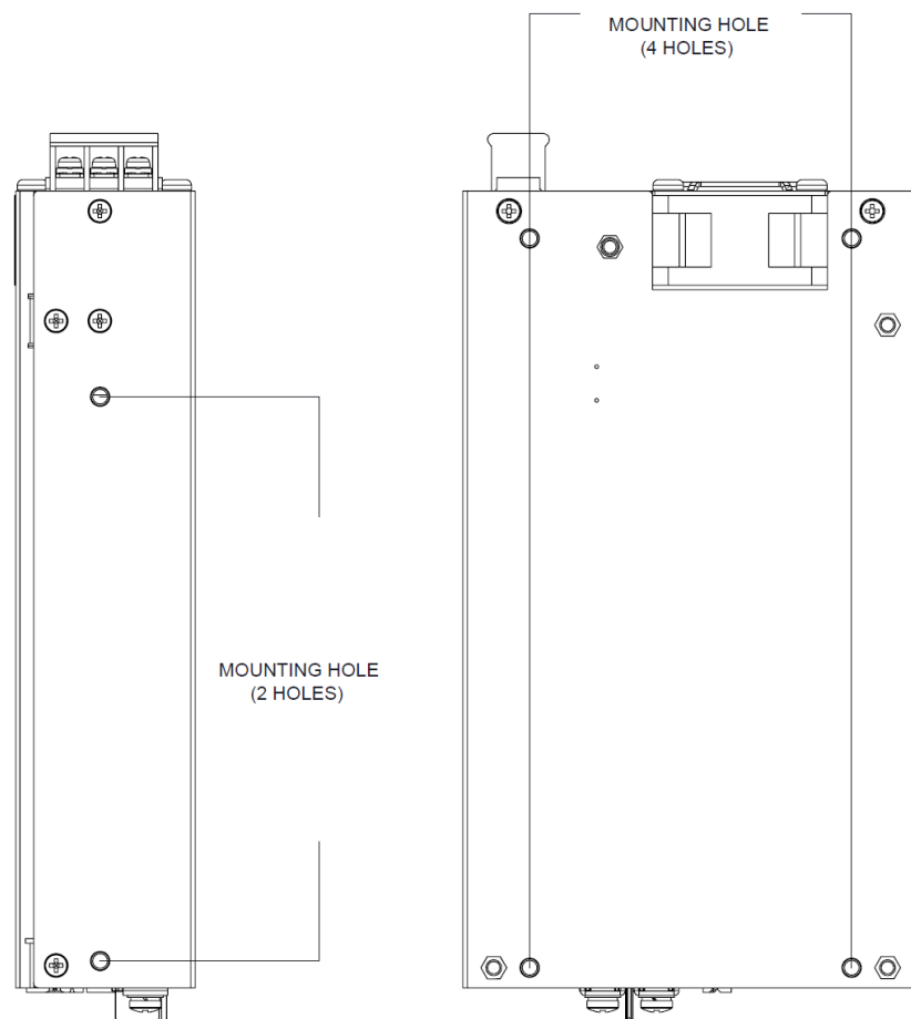
Fig. 13: Position of mounting holes
