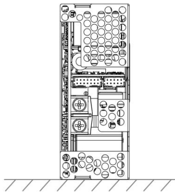
Fig. 11: Mounting on the right side
