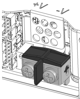
Fig. 8: Main DC Output terminal (CN101, CN102) – pin assignment
