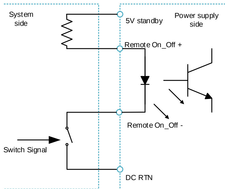
Fig. 20: Remote On_off connection
