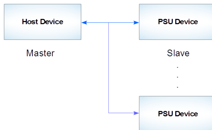
Fig. 1: I2C Topology
