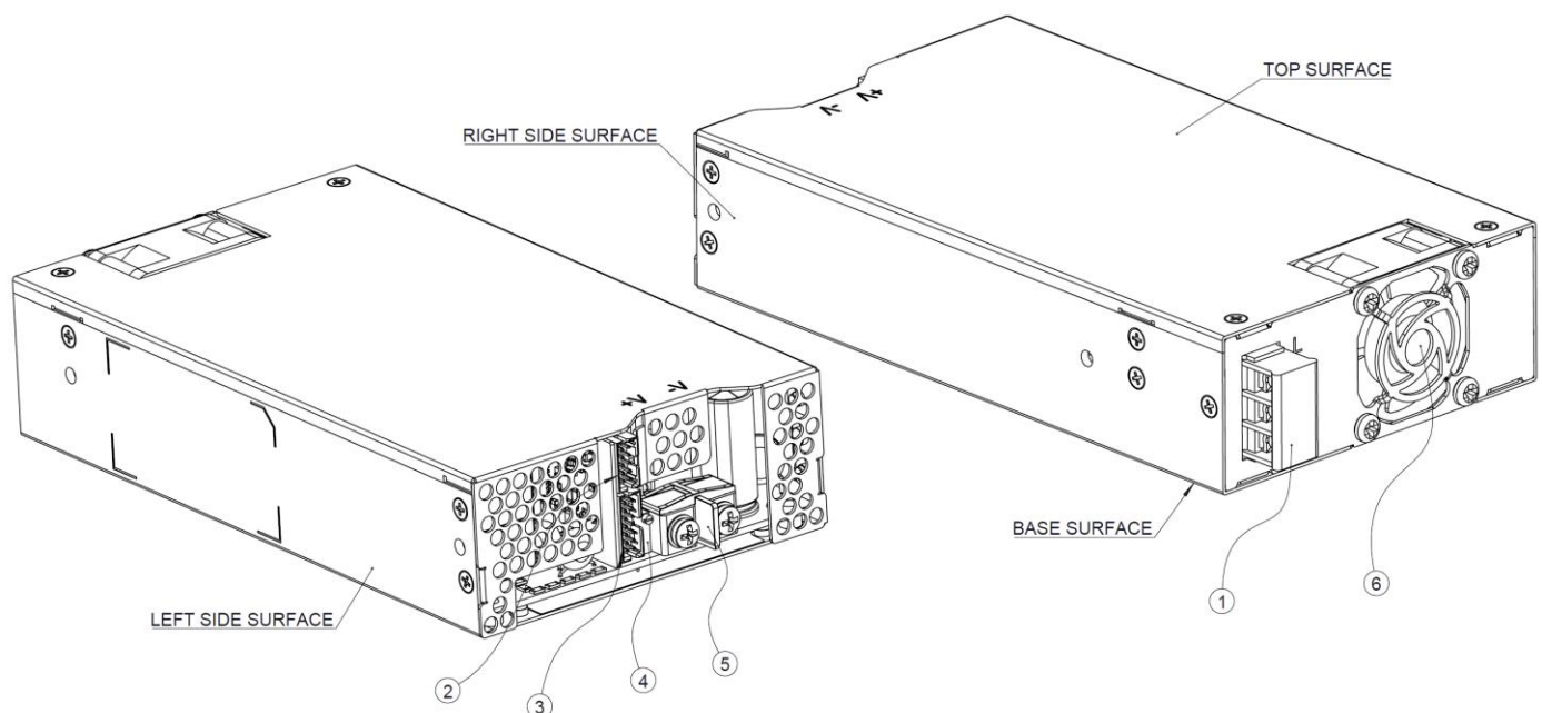
Fig. 1: Components of the PMS-XV750W1BTD series
