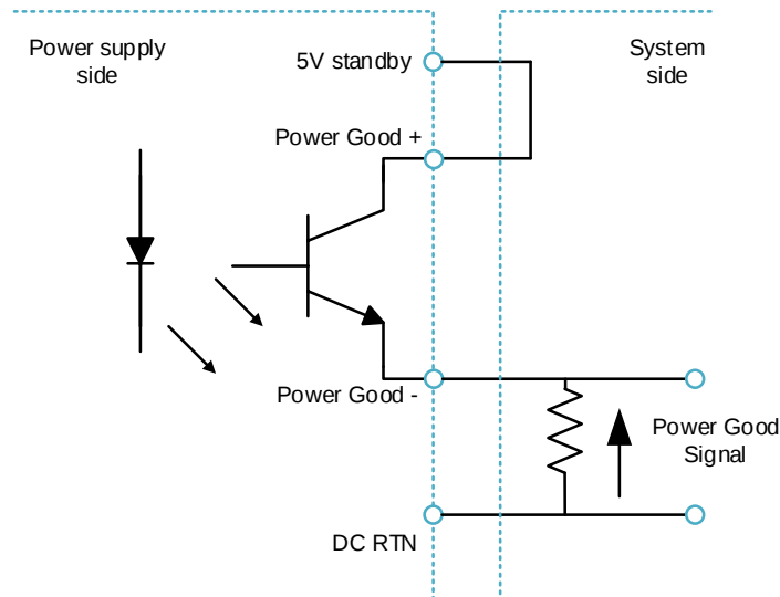
Fig. 21: Power good signal connection
