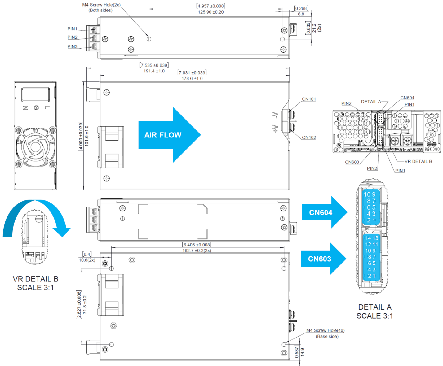
Fig. 14: Dimensional drawing PMS-XV750W1BDT
