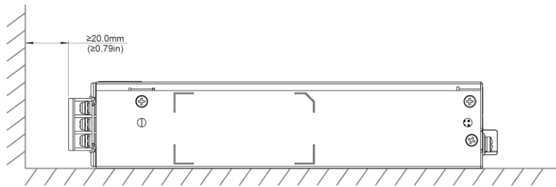
Fig. 9: Standard mounting orientation
