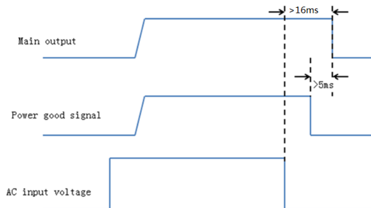
Fig. 22: Power good signal sequence
