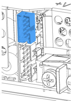
Fig. 3: Signal port and Auxiliary DC Output (CN604)
