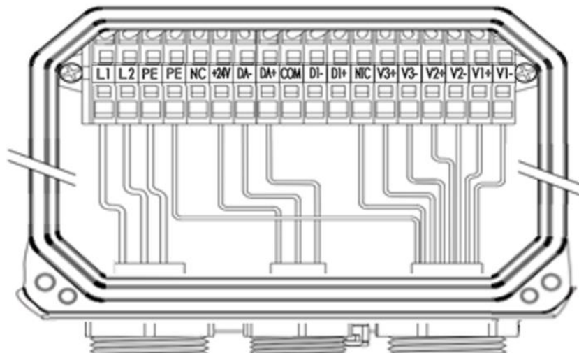
DALI Connection
