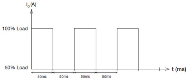
Figure 7. Dynamic Load
