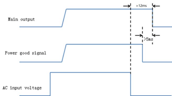
Figure 11. Power Good Time Sequence
