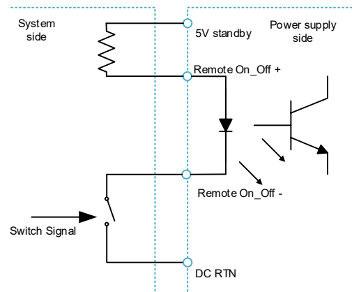
Figure 12. Remote On_Off Connection
