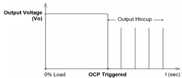
Figure 9. Hiccup at OLP/OCP
