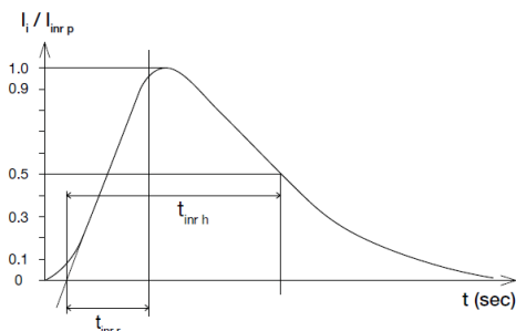
Fig. 7 Inrush Current
