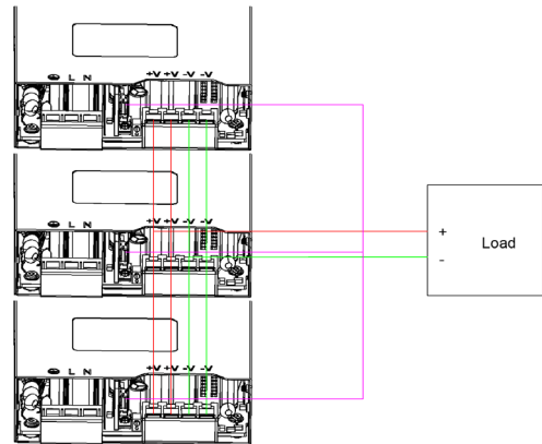
Fig. 10 Parallel Connection
