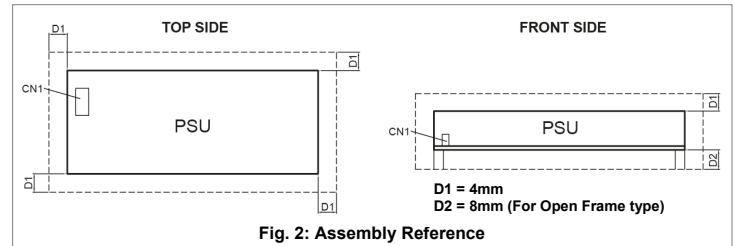
Fig. 2: Assembly Reference
