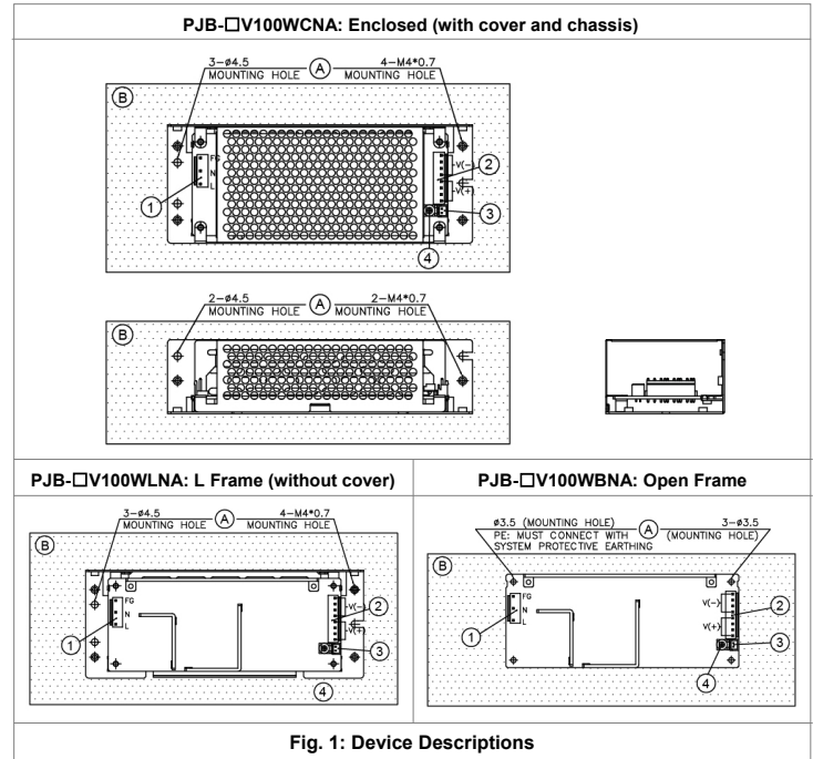
Fig. 1: Device Descriptions
