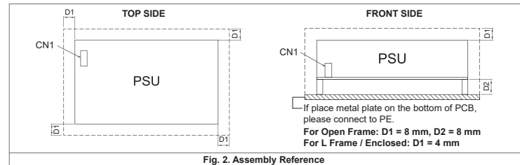
Fig. 2. Assembly Reference
