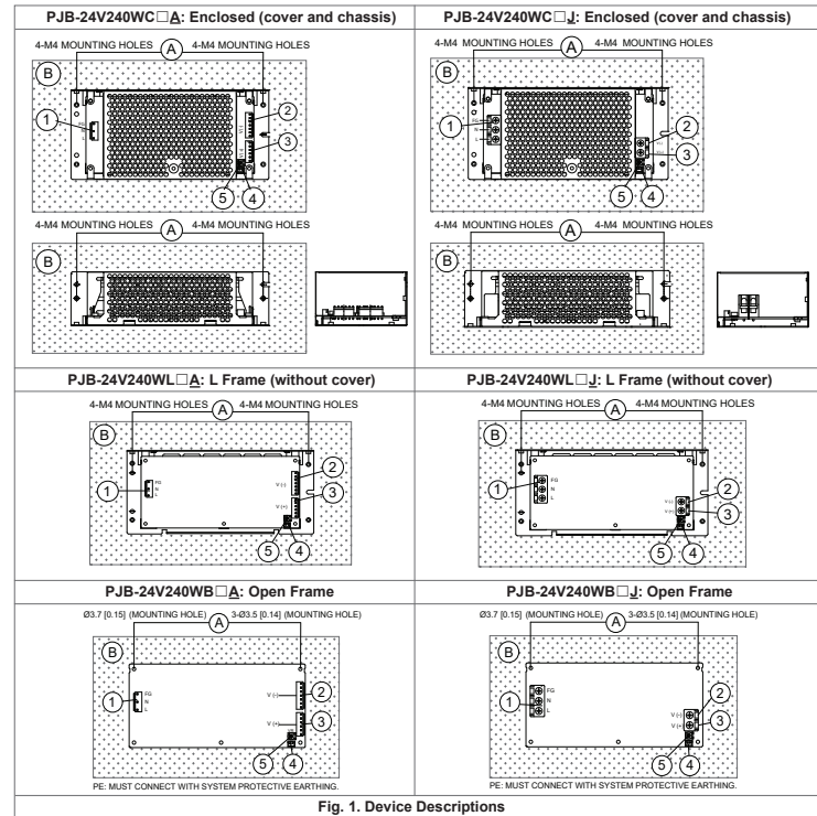
Fig. 1. Device Descriptions
