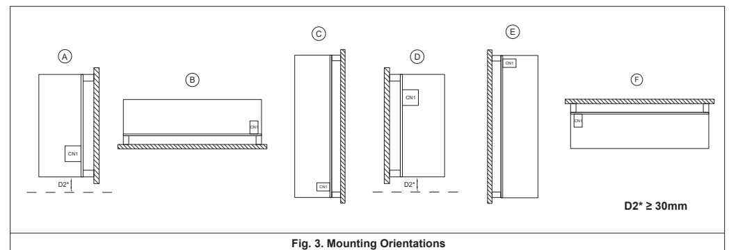
Fig. 3. Mounting Orientations
