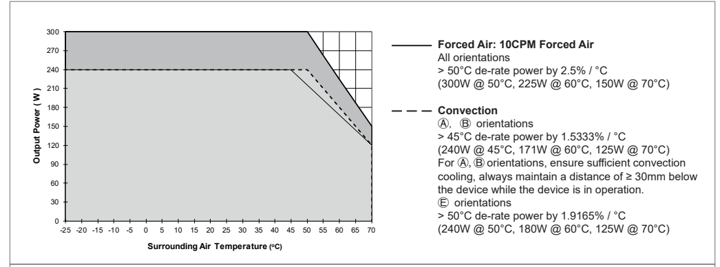
Fig. 4. Power Derating Curve
