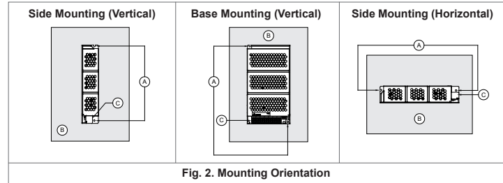
Fig. 2. Mounting Orientation
