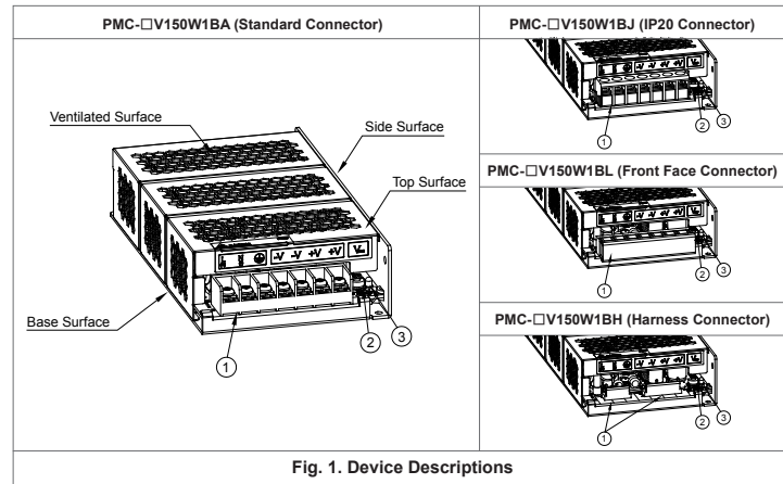
Fig. 1. Device Descriptions
