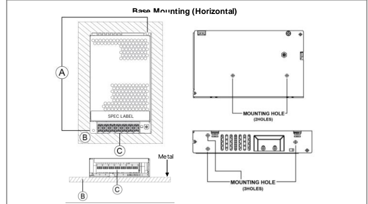
Fig. 3. Recommended Mounting Orientations & Mounting Hole Locations
