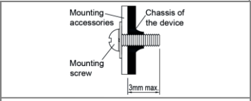
Fig. 5. Assembly Reference
