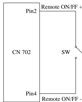
Fig. 20: Remote On_off connection
