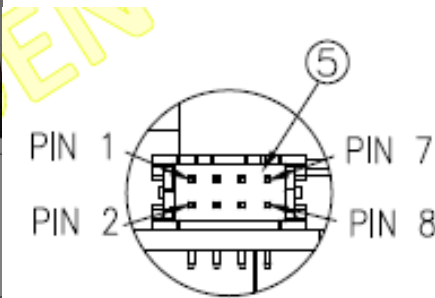
Fig. 3: Signal port and Auxiliary DC Output(CN702)
