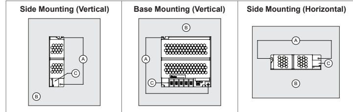
Fig. 2. Mounting Orientation
