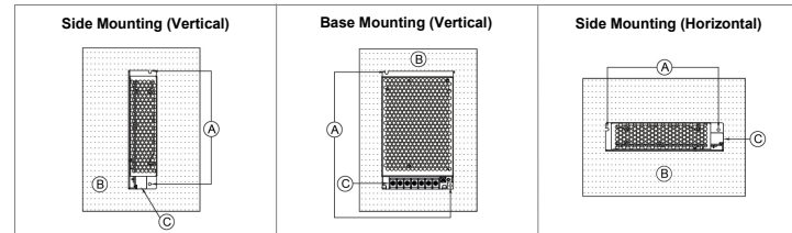
Fig. 2. Mounting Orientation
