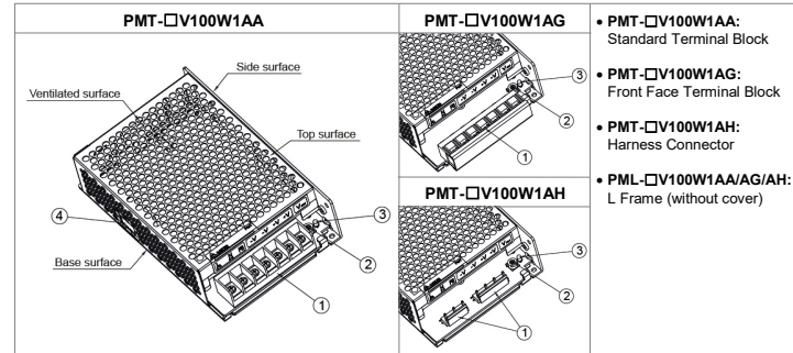
Fig. 1. Device Descriptions
