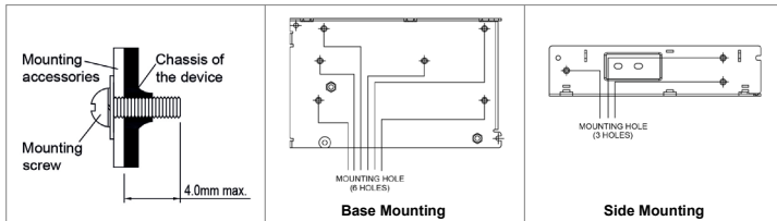
Fig. 4. Mounting Screw
