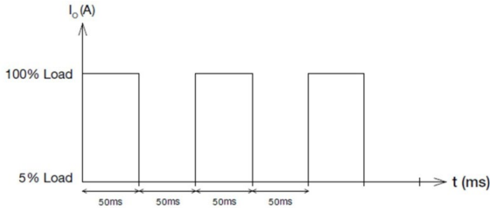
Figure 6. Dynamic Load
