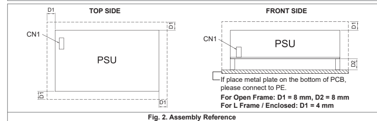
Fig. 2. Assembly Reference
