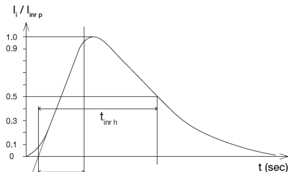
Figure 7. Inrush Current
