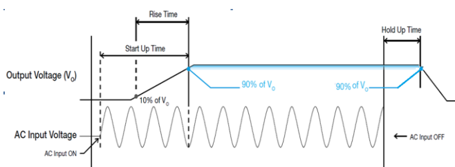
Figure 5. Time sequence
