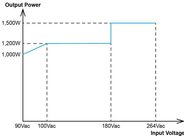
Fig. 4 De-rating for AC Input Voltage
