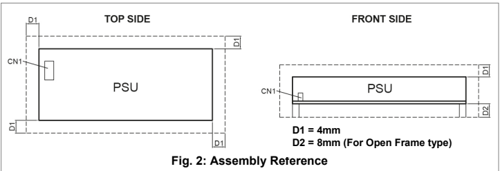
Fig. 2: Assembly Reference
