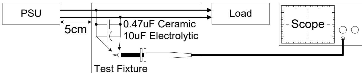
Fig. 22: Ripple and noise measurement circuit
