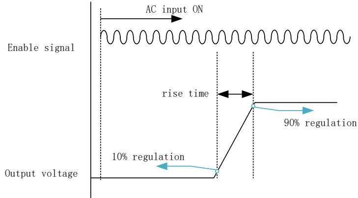
Fig. 20: Rise time sequence
