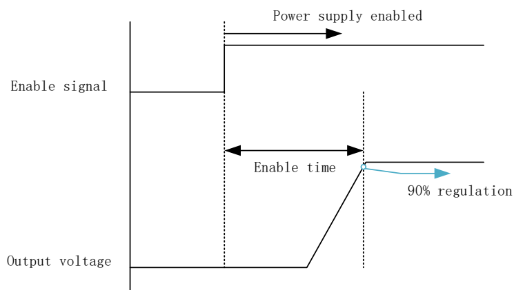
Fig. 19: Enable timing sequence
