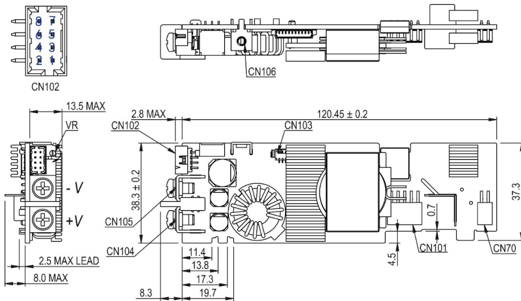
Fig. 6: Dimensional drawing Single Slot Module
