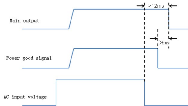
Fig. 26: Power good signal sequence
