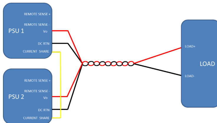
Fig. 29: Parallel connection without remote sense
