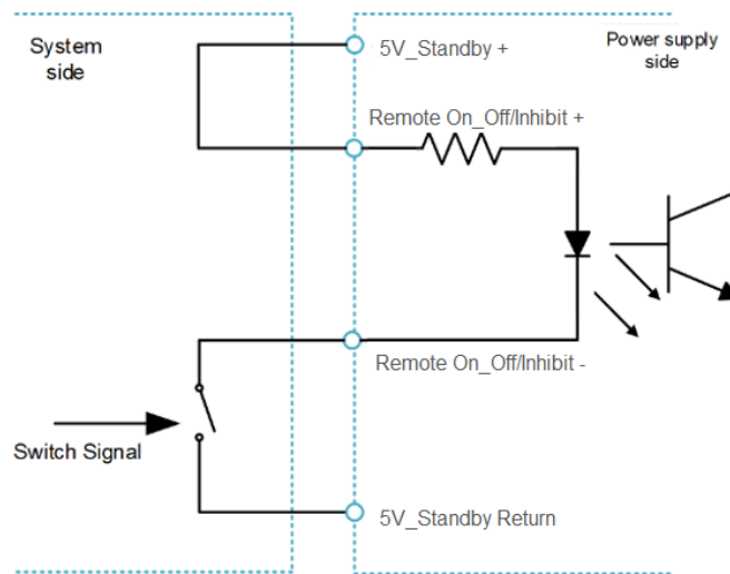
Fig. 24: Remote On_off connection
