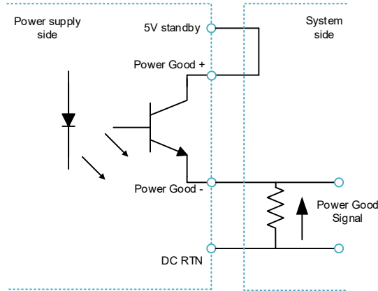
Fig. 25: Power good signal connection
