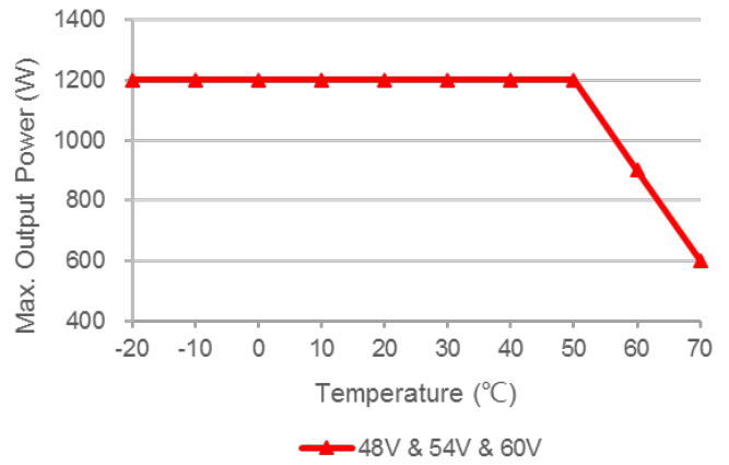
48V Module Max. Output Power Derating Curves
