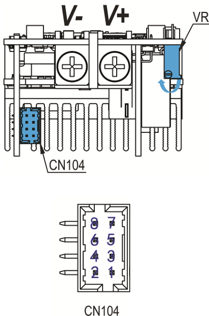
Fig. 16: -x2 Module connector
