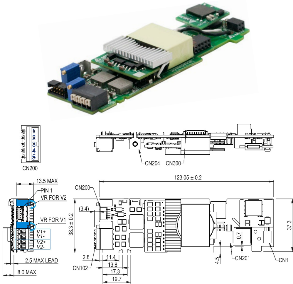
Fig. 8: Dimensional drawing Single Slot Dual Output Module
