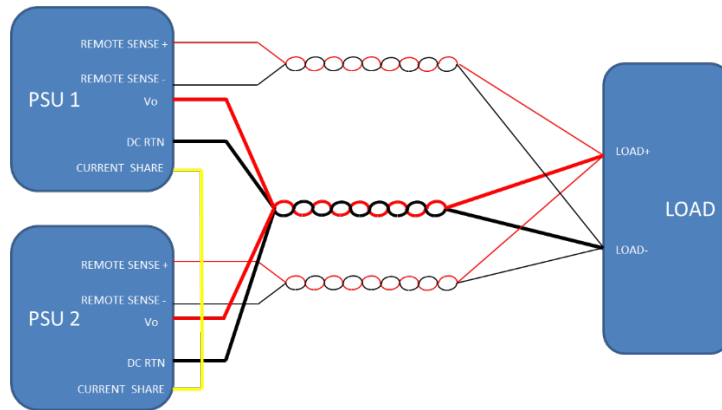
Fig. 28: Parallel connection with remote sense
