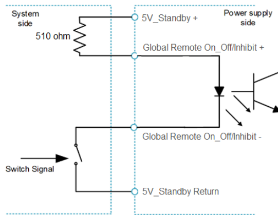
Fig. 31: Remote On_off connection
