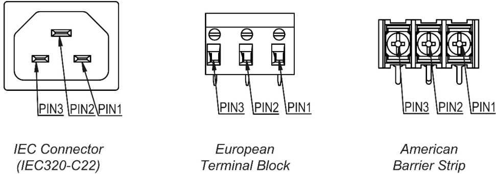
Fig. 13: AC Input Connector
