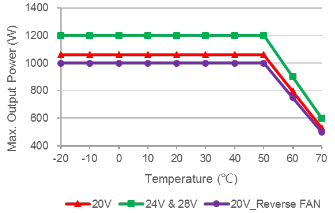
24V Module Max. Output Power Derating Curves
