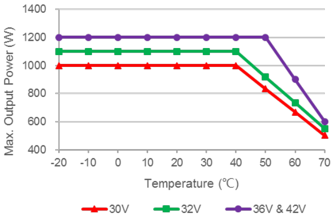
36V Module Max. Output Power Derating Curves
