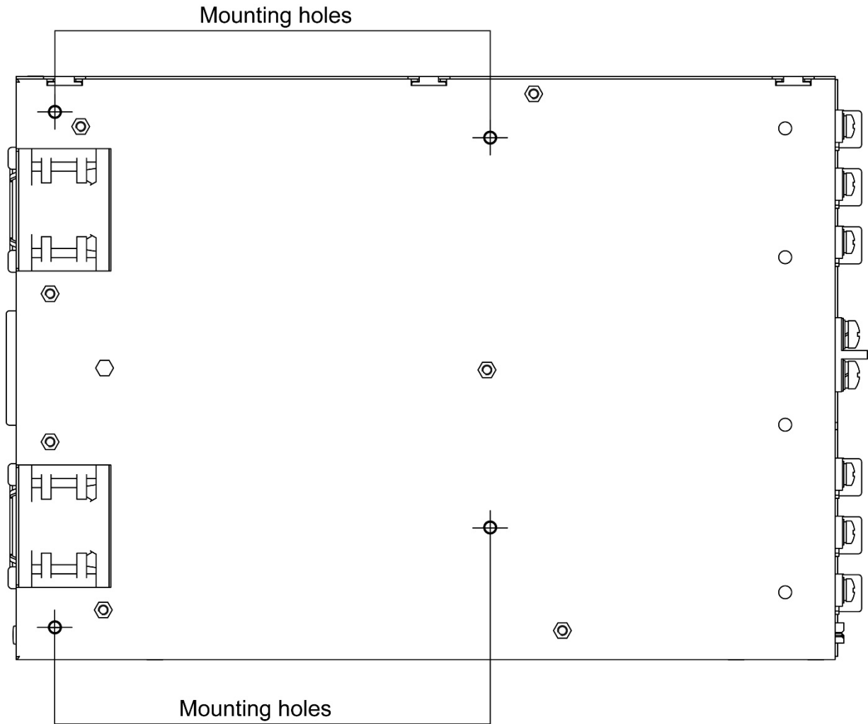
Fig. 4: Position of mounting holes
