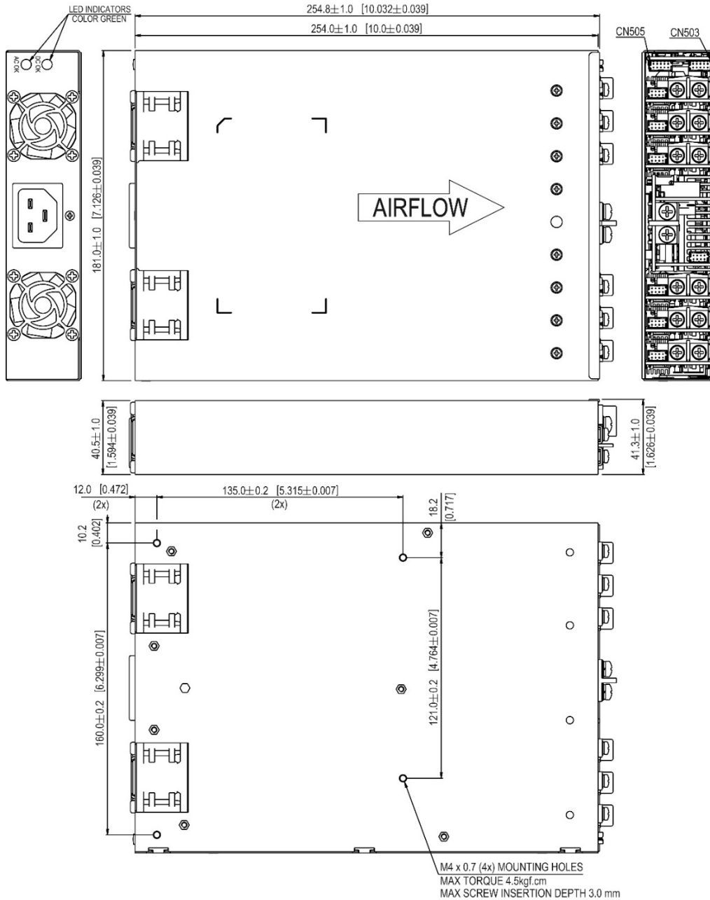
Fig. 5: Dimensional drawing MEG-3K0A
