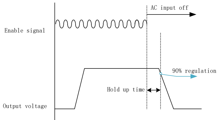
Fig. 21: Hold up time sequence
