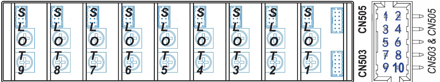
Fig. 14: Global Control Signals and Communications Connector
