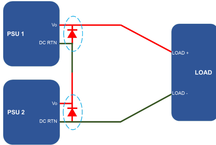
Fig. 30: Series connection with external reversed diode
