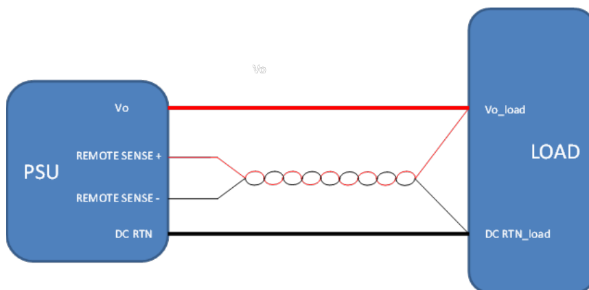
Fig. 27: Remote sense connection
