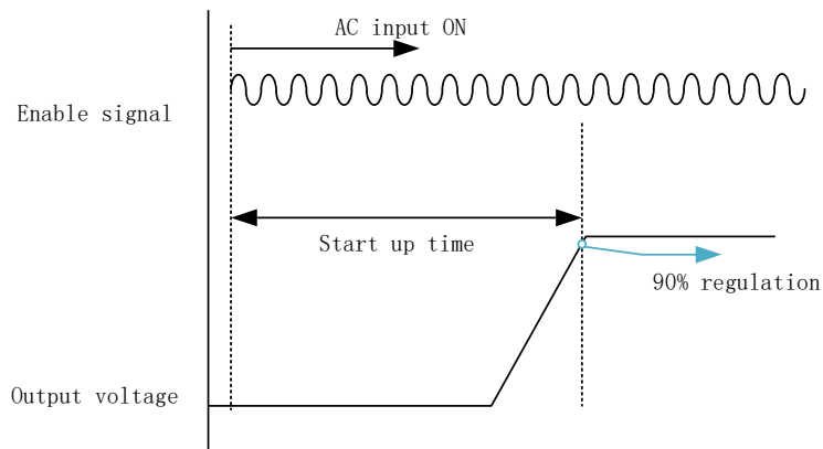
Fig. 18: Start-up timing sequence
